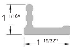
6914 PERIMETER TRIM
