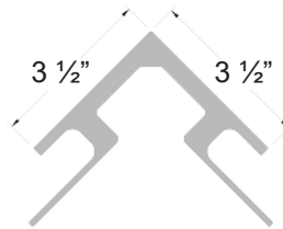
7910 3-1/2" OUTSIDE CORNER WITH FIN AND J-CHANNEL
