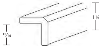
Coverage \frac{13}{16} " both directions
