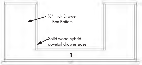
Bottom Pipe Clearance Drawer Box
