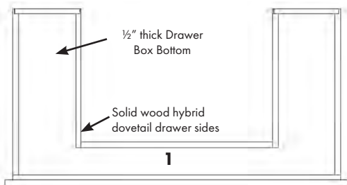
Bottom Pipe Clearance Drawer Box
