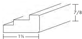
LRAIL Light Rail
