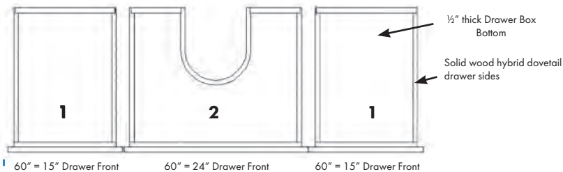
Standard Drawer Box Top & Bottom
