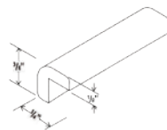
Outside Corner Molding
